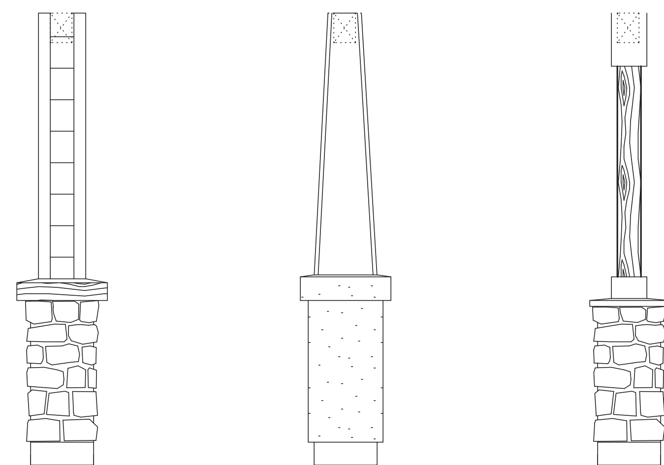
SQ. FRAMED COLUMN WITH STONE BASE TAPERED COLUMN WITH STUCCO BASE ROUGH SAWN POST WITH STONE BASE
