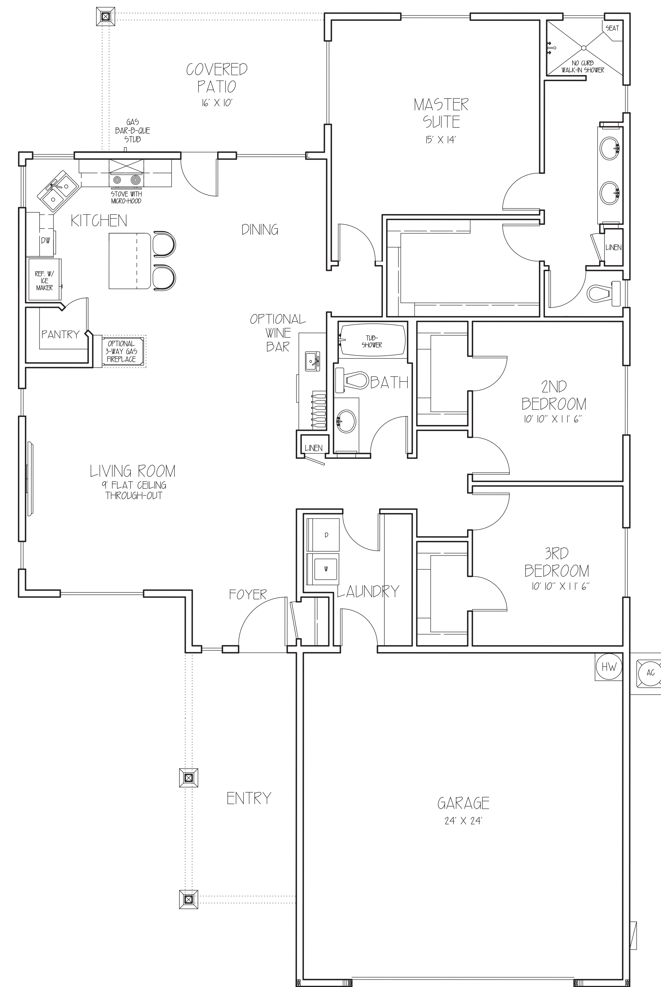
FLOOR PLAN
